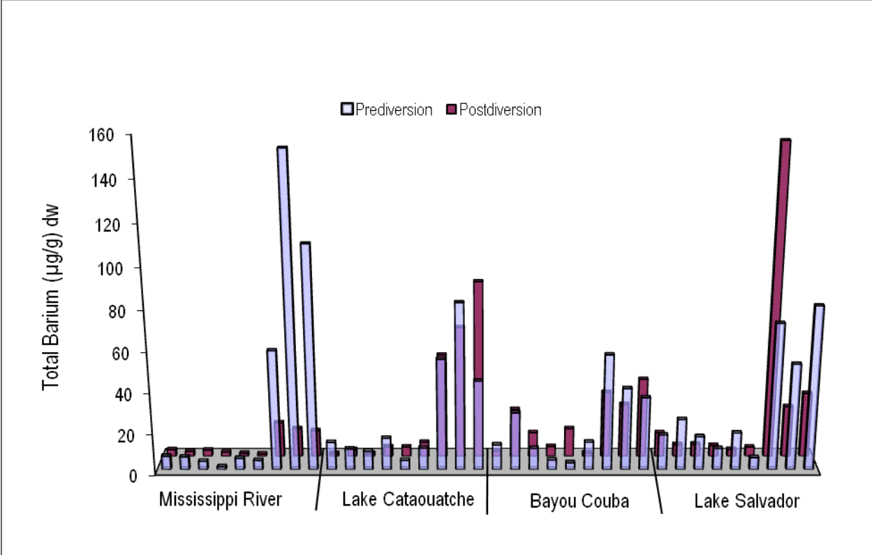
Figure 11B. Three-dimensional comparison of Davis Pond prediversion and postdiversion values for barium by dry weight (in micrograms per gram [ \mu\text{g/g} ]).
